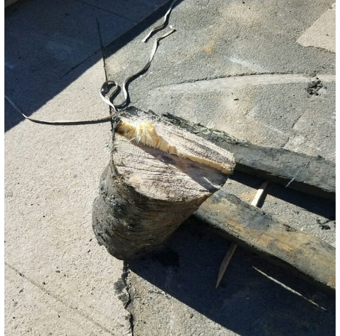
Sample condition of existing wood pile from D Street.
