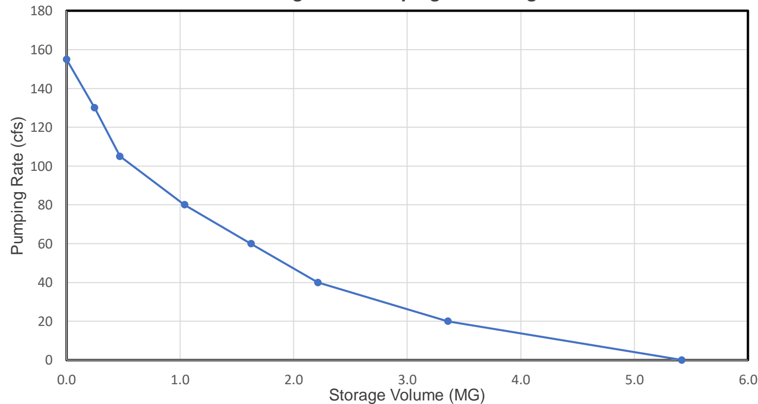
Figure 1: Pumping vs. Storage
