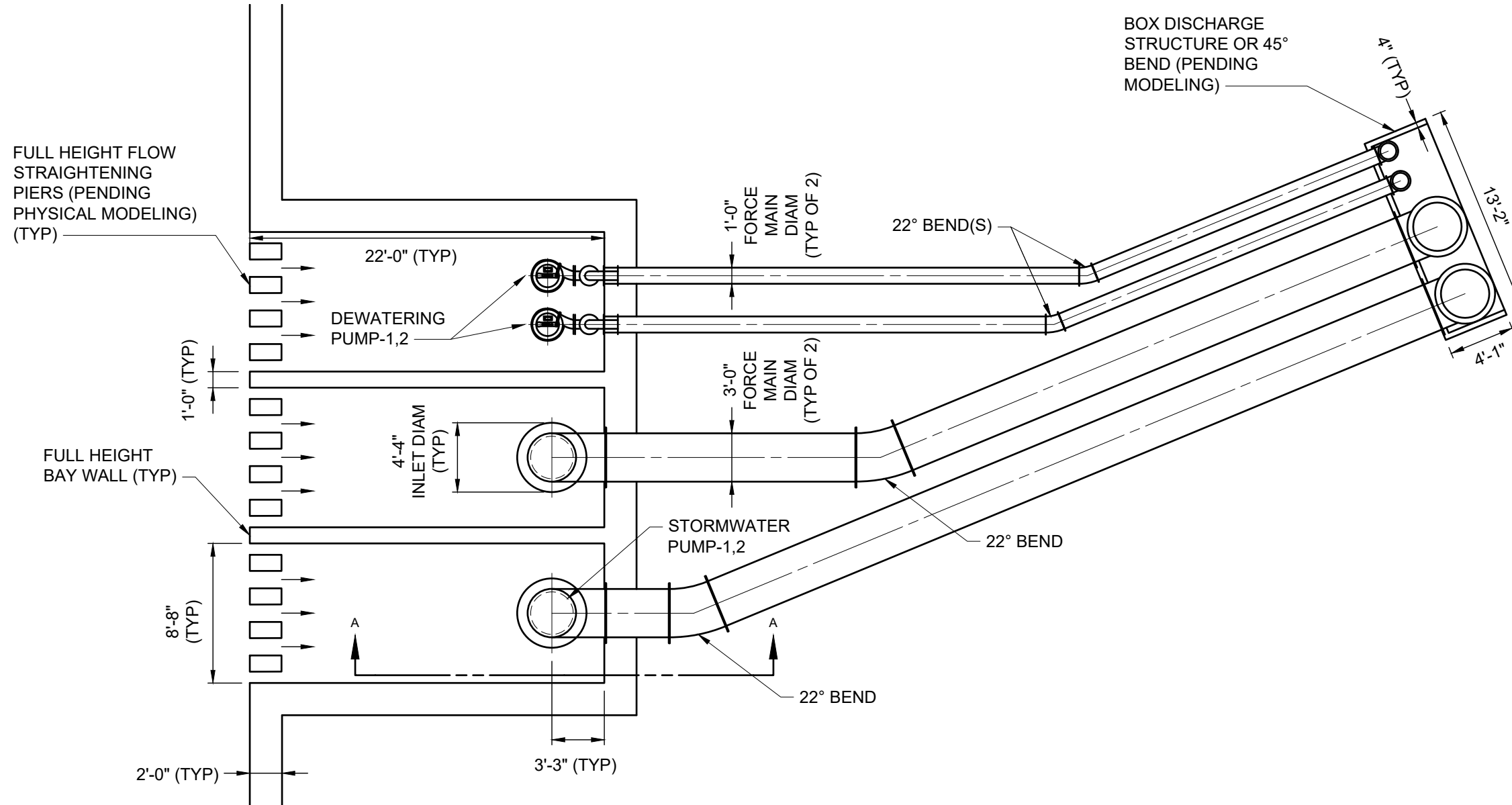
PUMP STATION PLAN SCALE: NTS
