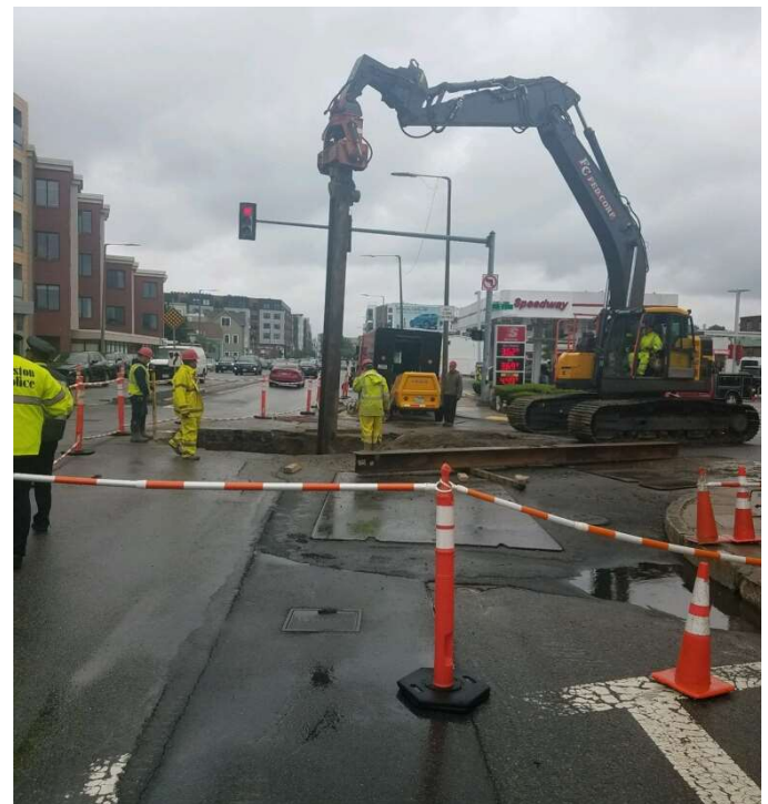
Support of Excavation on D Street
