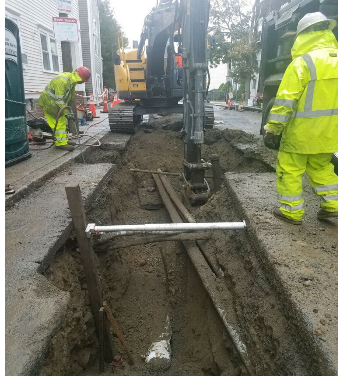
Trench Excavation of watermain in West Eighth Street
